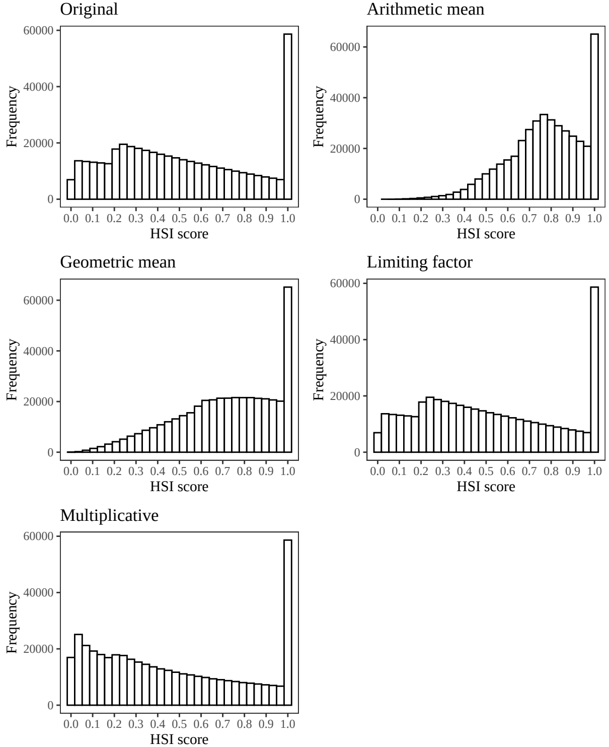
Figure 2. Empirical distributions of HSI scores for the stripedbassInlandRiv model using the original limiting factor model equation from Crance (1984), and an arithmetic mean, geometric mean, limiting factor, and multiplicative structure incorporating all SIV variables. Note differences in the y axis.
