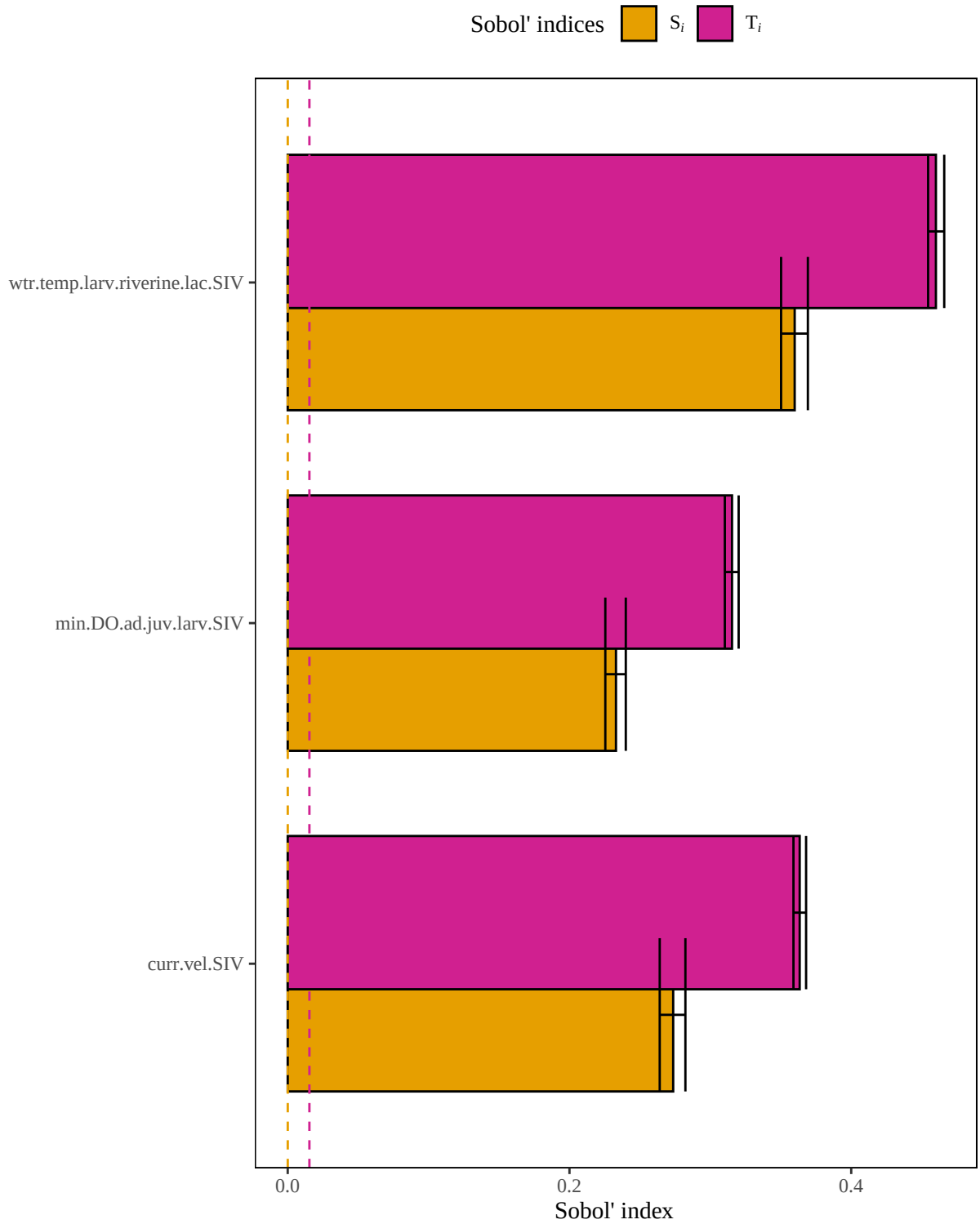
Figure 7. Results of a sensitivity analysis for the stripedbassInlandRiv model based on a multiplicative mean structure. Dashed lines represent baseline numerical approximation error for S_i and T_i ( i.e. , dummy variables).
