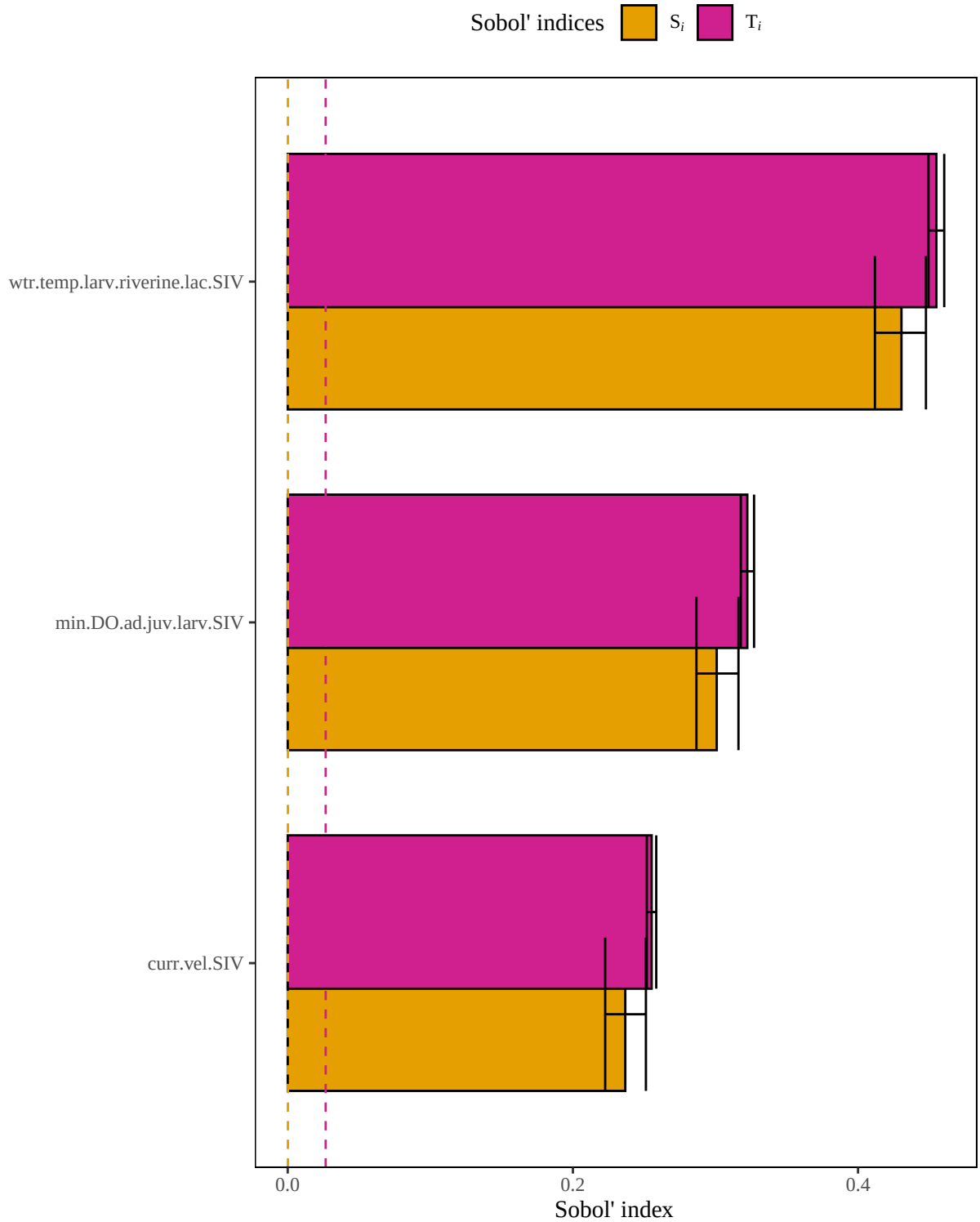
Figure 5. Results of a sensitivity analysis for the striped bass Inland Riv model based on a geometric mean structure. Dashed lines represent baseline numerical approximation error for S_i and T_i ( i.e. , dummy variables).
